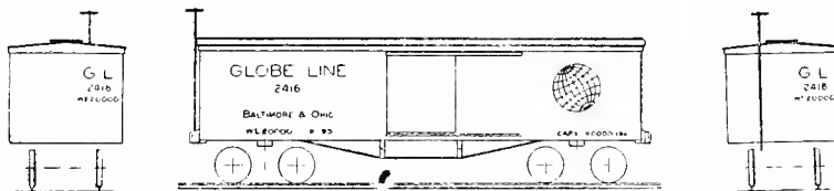
Figs. 5543-5545. MARKINGS FOR FAST FREIGHT LINE CARS. Recommended Practice, adopted in 1893.
